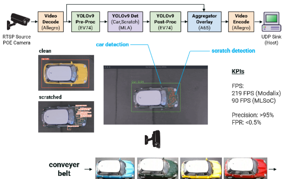
Car Scratch - Demo Architecture
